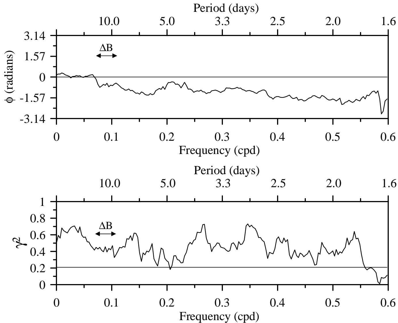
Coherence squared and phase between wind along 43T and the 1 st EOF time amplitude function for the NE Chukchi Sea in 1994-95. The solid horizontal line is the 90% significance level for \gamma^2 for the indicated bandwidth ( \Delta B ).
